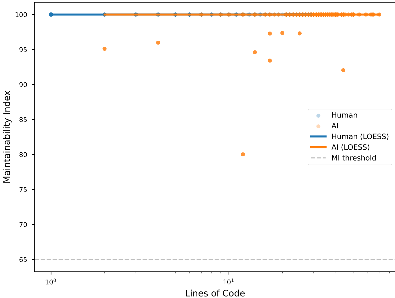
Maintainability Degradation with Solution Size
